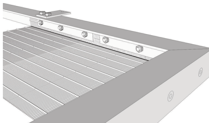
Mesh attachment to framework
